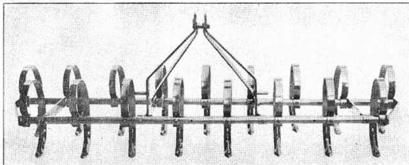
No. F128—Eight-foot 17-tooth Springtooth Harrow ready for Attachment to Tractor
